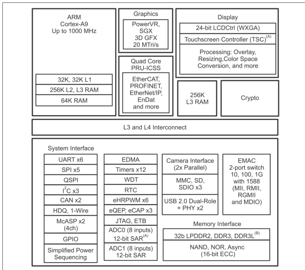
Figure 2 SITARA AM437X Block Diagram
