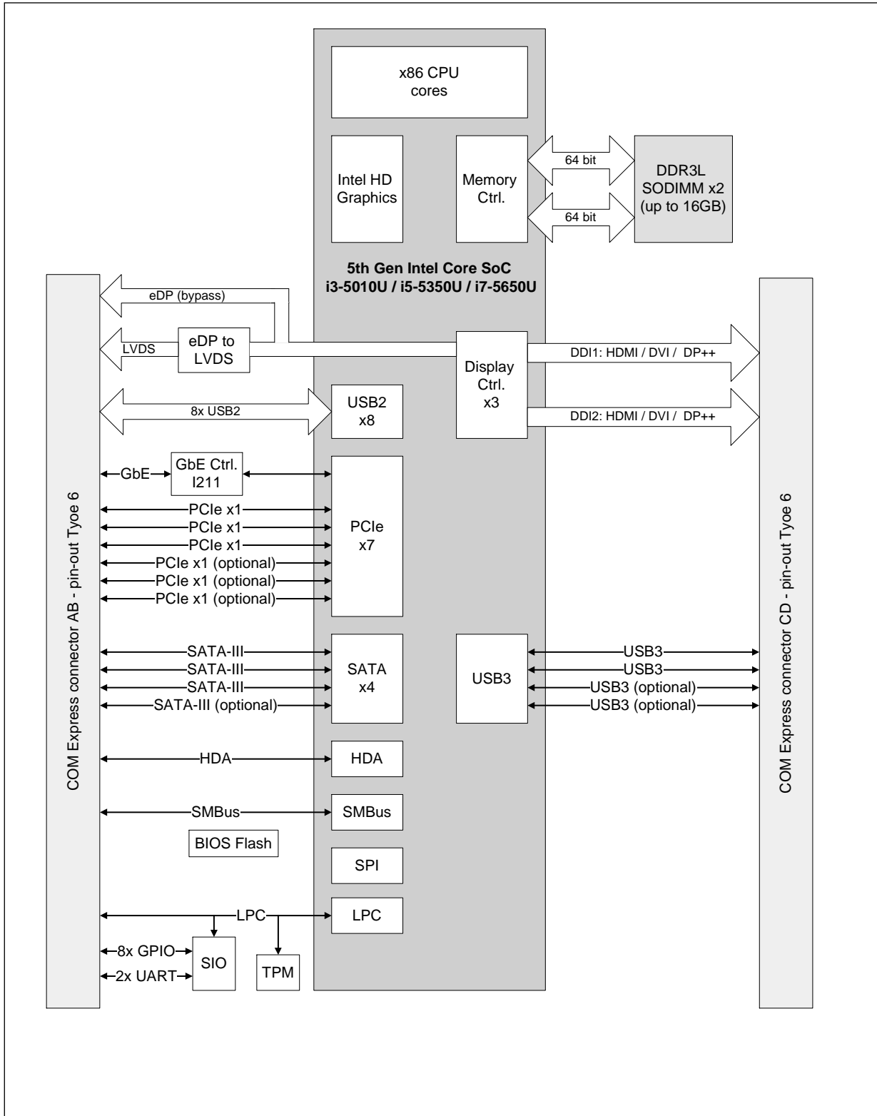
Figure 1 COMEX-IC50L Block Diagram
