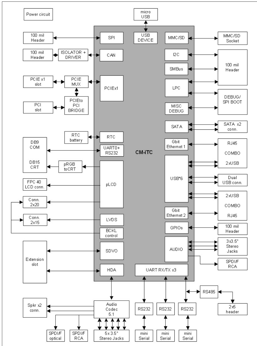
Figure 1 SB-iTC Block Diagram
