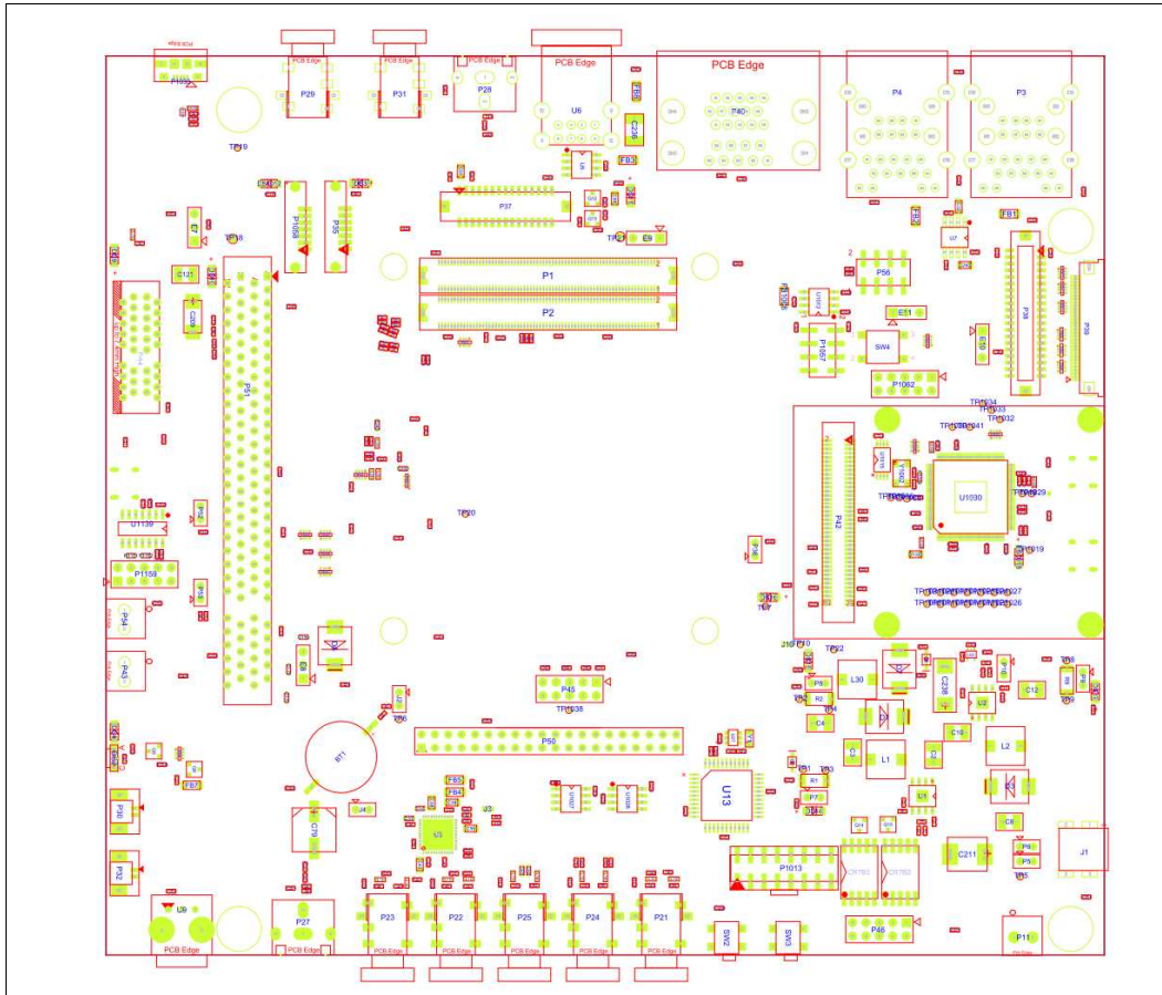
Figure 6 SB-iTC – Top View
