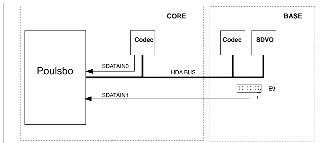
Figure 3 Audio Interface Block Diagram
