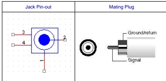
Figure 5 RCA Jack:
