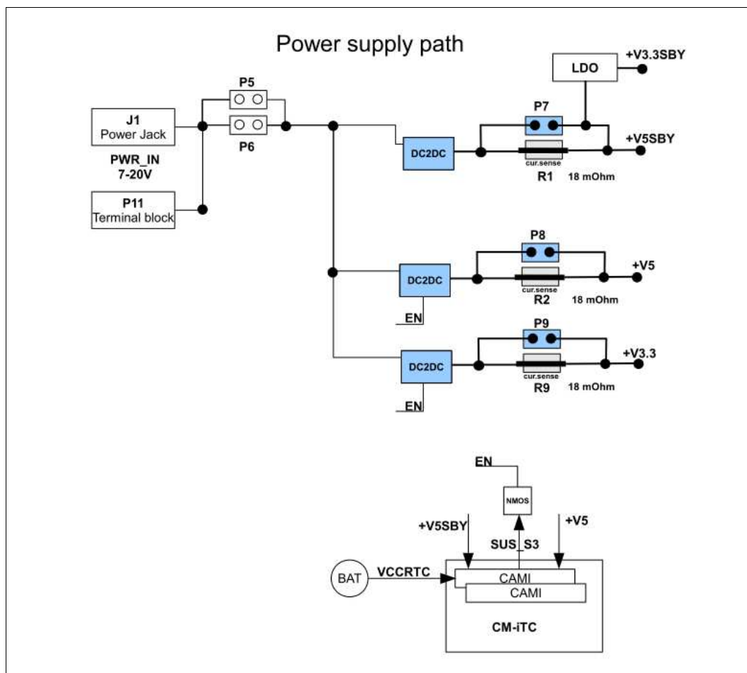
Figure 2 Power Supply Path
