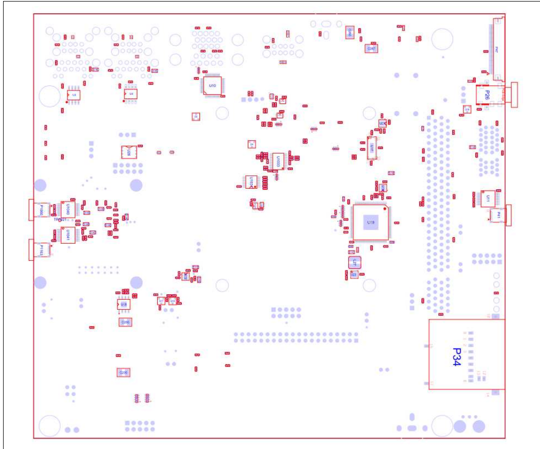
Figure 7 SB-iTC – Bottom View
