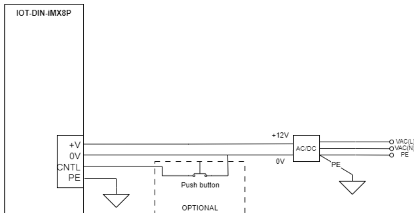
Figure 4 power connector typical connection
