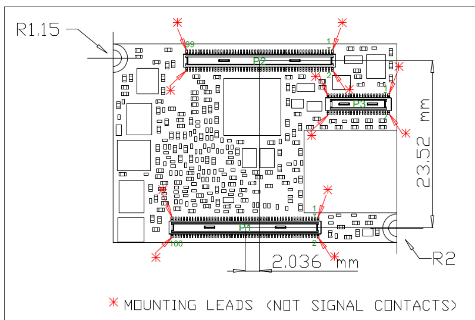
Figure 4 UCM-iMX95 bottom
