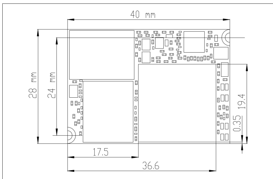
Figure 4 UCM-iMX95 bottom
