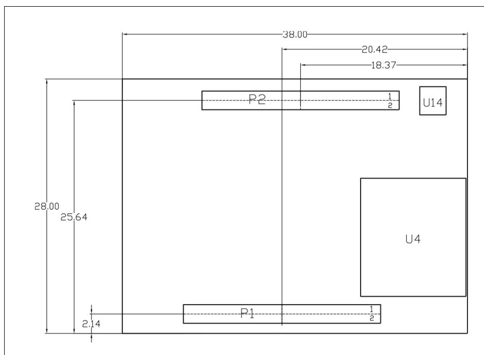
Figure 4 UCM-iMX8M-Mini bottom
