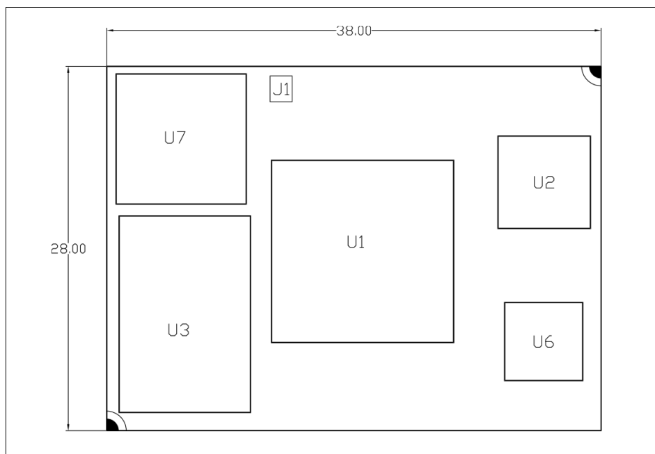
Figure 4 UCM-iMX8M-Mini bottom
