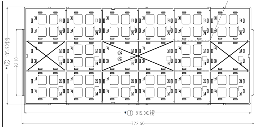
Figure 5 MCM-iMX95 tray
