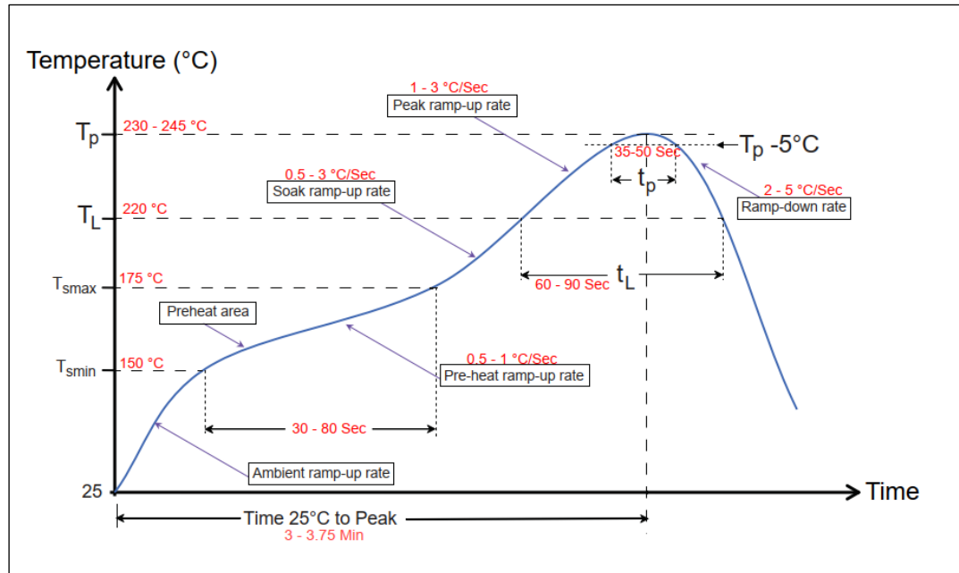
Figure 6 Reference reflow profile
